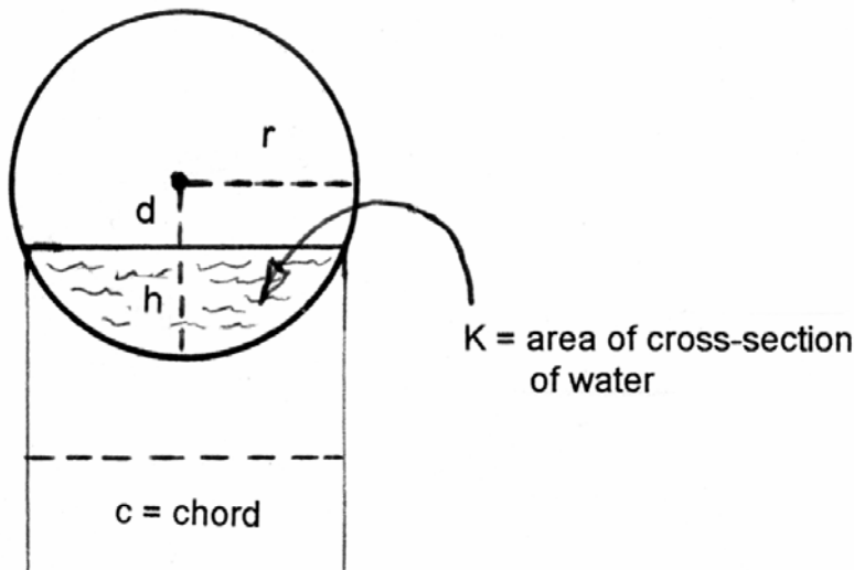
Figure A4.1. A sketch of the cross-section of the cylindrical culvert. The various symbols are shown, as used in formulae for calculating depths and cross-sections.
